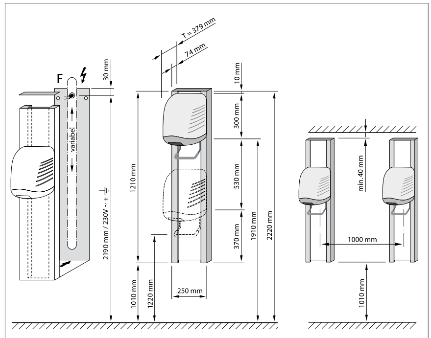
Warm-air shower Vendaval fixed device Warm-air shower Vendaval V/S height adjustable
