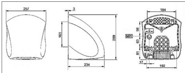
Ultronic W Hand dryer
