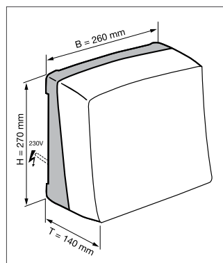
Hand dryer AirStream 2000
