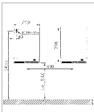
Hand dryer WP 1100
