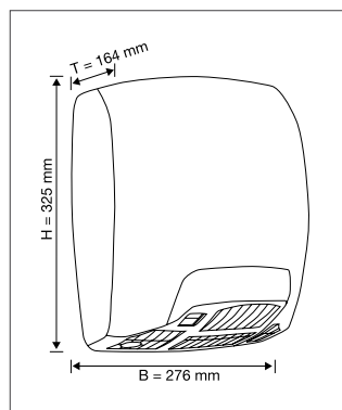
Hand dryer MFLW 2
